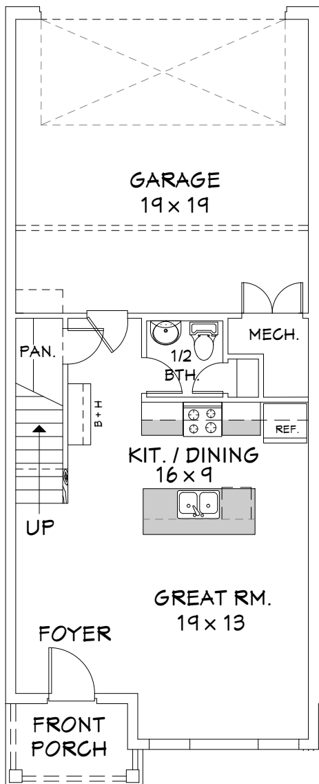
1 st Level Floorplan
