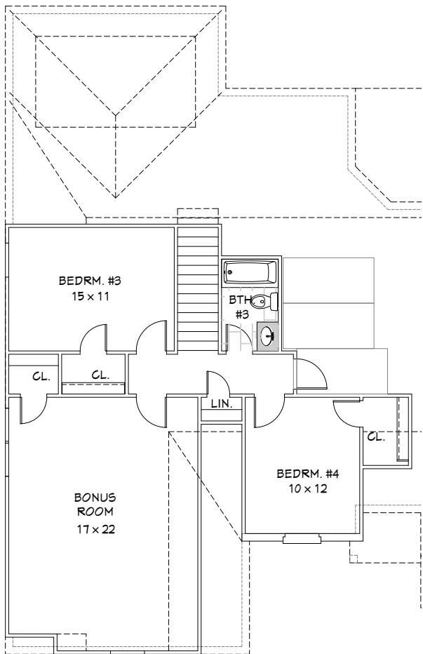
Second Level Floor Plan
