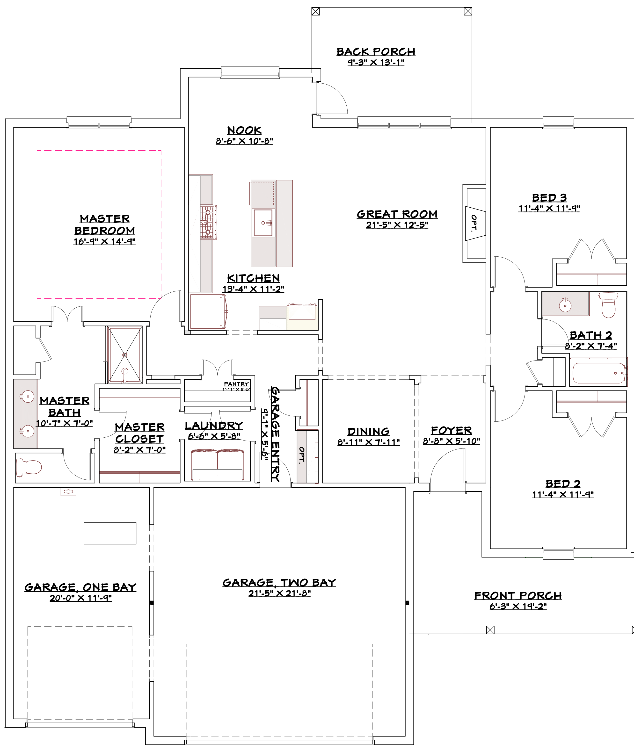
FIRST FLOOR
